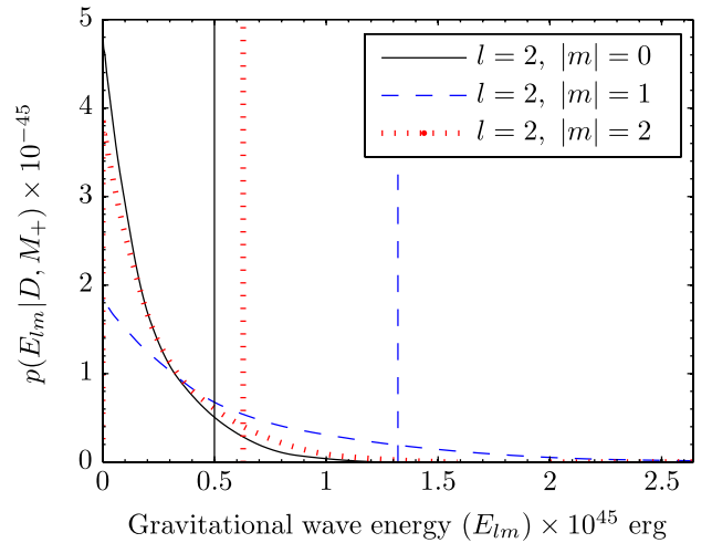
FIG. 4 (color online). The posterior probability density distributions and upper limits on the total gravitational-wave energy in the form of ring-downs, assuming only a single harmonic (i.e. value of |m| ) is excited. The upper limits for each harmonic are shown as the vertical lines in the figure. The numerical values of the 90% confidence upper limits can be found in Table IV. The l = 2 , |m| = 0 posterior is shown as the solid black line, the dashed curve (blue in the online version) shows the l = 2 , |m| = 1 posterior, and the l = 2 , |m| = 2 posterior is shown as the dotted curve (red in the online version).
