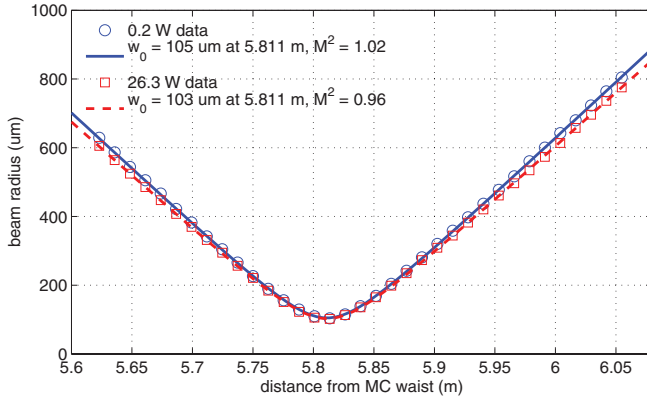
FIG. 9. Profile at high and low powers of a pick-off of the beam transmitted through the MC. The precision of the beam profiler is \pm 5\% . Within the error of the measurement, there are no obvious degradations.
