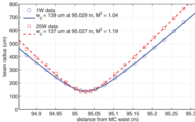
FIG. 10. Faraday isolator thermal lensing data. With 25 W into the Faraday isolator (corresponding to 50 W in double pass), the beam has a steeper divergence than a pure TEM 00 beam, indicating the presence of higher order modes. Errors are \pm 5.0\% for each data point.
