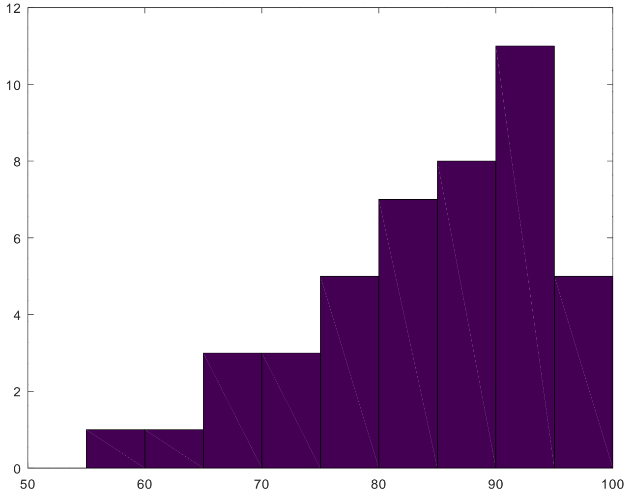
Exam 2 Fall 2019 Distribution (mean=84.75, std=10.0)
