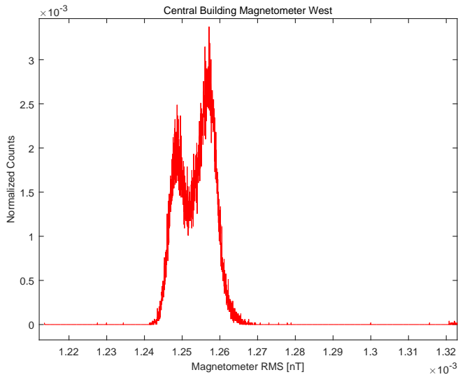
Figure 4: Binned, normalized distribution of Power-OFF RMS for Central Building Magnetometer West. This distribution was computed for a day of rms trend data. Note that the distribution is not Rayleigh distributed.
