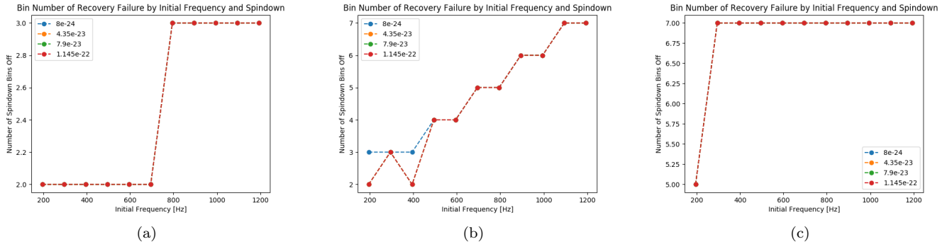
FIG. 5: This figure represents three different cases of the same source recovery test. Each figure gives the number of spindown bins by which the correction parameters deviate from the source to such an extent that the source parameters are no longer recovered by the traditional FrequencyHough procedure described in Section III. Figure 5a is the case T_{FFT} = 2 s, Figure 5b is the case T_{FFT} = 4 s, and Figure 5c is the case T_{FFT} = 8 s. All three figures were generated with from a 600 second duration signal with braking index 7 in real detector noise from shortly after GW170817. The spindown for each case is the maximum spindown for the T_{FFT} in question.
