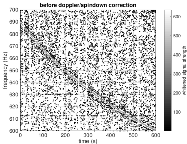
FIG. 1: A 600 second duration peakmap constructed from 2 second FFTs for a source with f_0 = 690 Hz, \dot{f}_0 = -0.25 Hz/s, and n = 7 in white noise. The frequency evolution for this set of source parameters over the 600 seconds is clearly visible and shows the signal decreasing by approximately 90 Hz.
