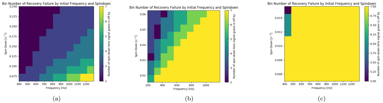
FIG. 4: This figure represents three different cases of the same source recovery test. Each figure gives the number of spindown bins by which the correction parameters deviate from the source to such an extent that the source parameters are no longer recovered by the traditional FrequencyHough procedure described in Section III. Figure 4a is the case T_{FFT} = 2 s, Figure 4b is the case T_{FFT} = 4 s, and Figure 4c is the case T_{FFT} = 8 s. All three figures were generated with from a 600 second duration signal with braking index 7 in real Livingston detector noise from shortly after GW170817. The spindown range for each case reflects the range for which the T_{FFT} in question is best suited.
