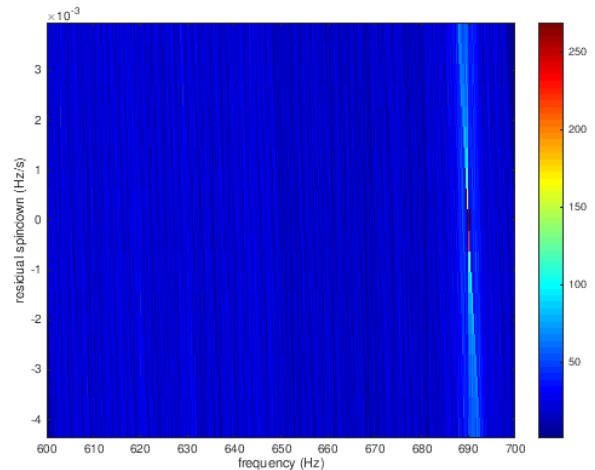
FIG. 3: This figure shows an example of a Hough map, which shows points of intersection of the lines described in III. This plot was generated using corrected 600 second duration peakmap constructed from 2 second FFTs for a source with f_0 = 690 Hz, \dot{f}_0 = -0.25 Hz/s, and n = 7 in white noise.
