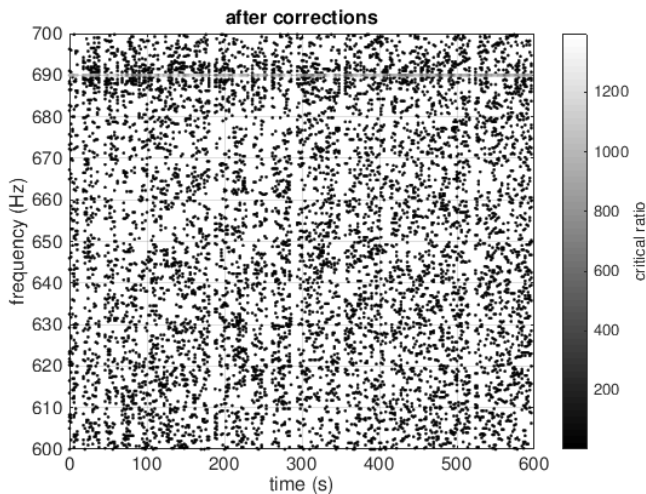
FIG. 2: A 600 second duration peakmap constructed from 2 second FFTs for a source with f_0 = 690 Hz, \dot{f}_0 = -0.25 Hz/s, and n = 7 in white noise. The signal in this case has been Doppler and spindown corrected using Equation 3, so the signal appears monochromatic at its initial frequency of 690 Hz.
