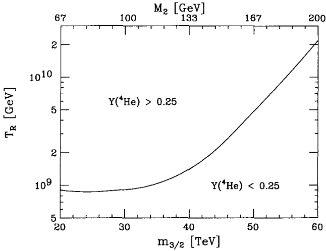
Fig. 7. The upper bound on the reheat temperature as a function of the gravitino mass m_{3/2} and the corresponding Wino mass M_2 . The observational limit upper limit on the primordial helium abundance is Y(^4\text{He}) < 0.25 . Therefore, the region above the line is excluded, and an upper bound on T_R results.
