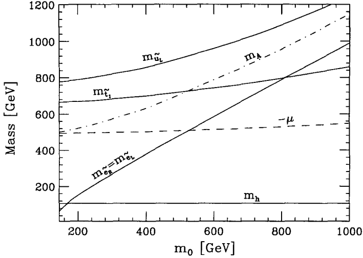
Fig. 1. Masses of several states in the supersymmetric spectrum as a function of m_0 with m_{3/2} = 36 TeV, \tan \beta = 5 , and \mu < 0 . The gaugino masses for this choice are M_1 = 333 GeV, M_2 = 119 GeV, and M_3 = 850 GeV.
