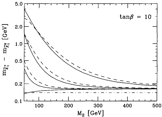
Fig. 3. The mass splitting as a function of M_2 for \tan\beta = 10 . The solid curves, from top to bottom, represent \mu = 2M_2 , \mu = 3M_2 , \mu = 5M_2 , and \mu = \infty . The dashed curves are the same except for the opposite sign of \mu . The dot-dashed curve is the charged pion mass m_{\pi^\pm} .
