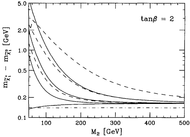
Fig. 2. The mass splitting as a function of M_2 for \tan\beta = 2 . The solid curves, from top to bottom, represent \mu = 2M_2 , \mu = 3M_2 , \mu = 5M_2 , and \mu = \infty . The dashed curves are the same except for the opposite sign of \mu . The dot-dashed curve is the charged pion mass m_{\pi^\pm} .
