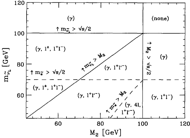
Fig. 6. Signatures of the AMSB scenario at LEP2. Each blocked region has a unique mass hierarchy among \tilde{\nu}_L , \tilde{e}_L and M_2 , and therefore leads to different signatures which are contained within the parenthesis. The meaning of “( \gamma )”, for example, is e^+e^- \rightarrow \gamma\tilde{W}^+\tilde{W}^- \rightarrow \gamma + \tilde{E} . We assume, as is justified by EWSB analysis, that M_2 is very close to the mass of the nearly degenerate lightest charginos and neutralino. The mass splitting between m_{\tilde{\nu}_L} and m_{\tilde{e}} is due to a hypercharge D -term, and its value is calculated with \tan\beta = 3 for this figure.
