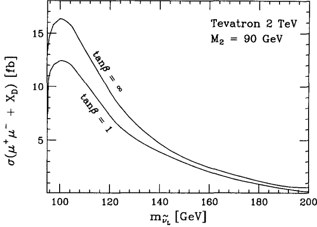
Fig. 4. Dilepton signal with at least one displaced vertex from smuon and sneutrino production at the Fermilab Tevatron with 2 TeV center of mass energy and M_2 = 90 GeV. Acceptance cuts of the leptons and efficiencies are described in the text. The different curves are for \tan \beta = 1 , which makes m_{\tilde{\mu}_L} = m_{\tilde{\nu}_L} , and for \tan \beta = \infty which maximizes the hypercharge D -term splitting such that m_{\tilde{\mu}_L}^2 = m_{\tilde{\nu}_L}^2 + m_W^2 . With 10 \text{ fb}^{-1} the Tevatron will record more than 10 such events for each lepton flavor if m_{\tilde{\nu}_L} < 185 GeV.
