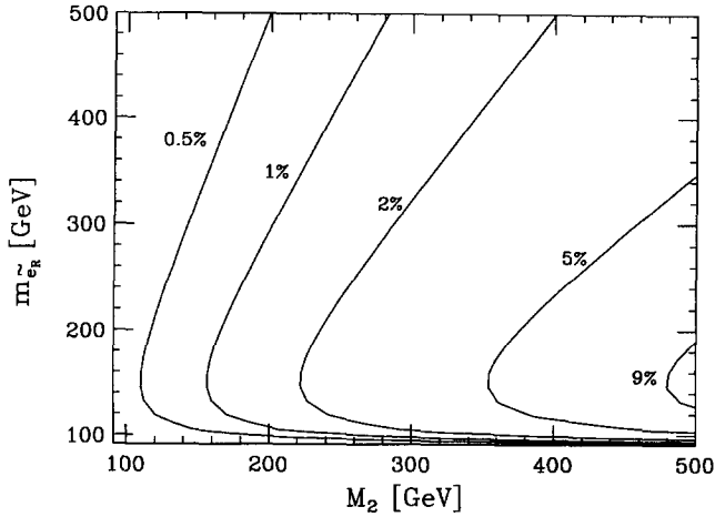
Fig. 5. Contours of 100\% \times (m_{\tilde{e}_L} - m_{\tilde{e}_R})/m_{\tilde{e}_R} in the M_2 - m_{\tilde{e}_R} mass plane with large \tan\beta , which maximizes the mass splitting.
