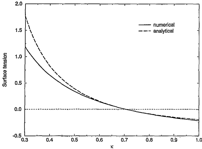
FIG. 4. Dimensionless surface tension \bar{\sigma}_{ns} as a function of the Ginzburg-Landau parameter \kappa for 0.3 < \kappa < 1.0 . The solid line is the numerical result, and the dashed line is the asymptotic expansion about \kappa = 1/\sqrt{2} given in Eq. (3.8).
