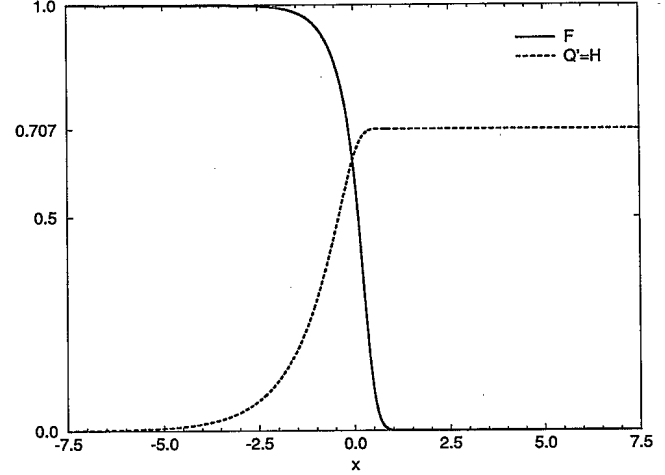
FIG. 2. Magnitude of the order parameter F and the magnetic field H for \kappa = 10 , which corresponds to a type-II superconductor. Lengths are in units of the penetration depth.
