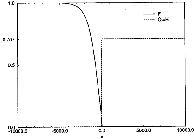
FIG. 1. Magnitude of the order parameter F and the magnetic field H for \kappa = 10^{-3} , which corresponds to a type-I superconductor. Lengths are in units of the penetration depth.
