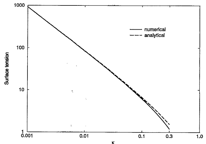
FIG. 3. Dimensionless surface tension \bar{\sigma}_{ns} as a function of the Ginzburg-Landau parameter \kappa for 10^{-3} < \kappa < 0.3 . The solid line is the numerical result, and the dashed line is the asymptotic expansion for \kappa \ll 1 given in Eq. (3.8).
