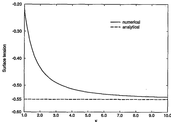
FIG. 5. Dimensionless surface tension \bar{\sigma}_{ns} as a function of the Ginzburg-Landau parameter \kappa for 1.0 < \kappa < 10.0 . The solid line is the numerical result, and the dashed line is the limiting value for \kappa \gg 1 given in Eq. (3.8).
