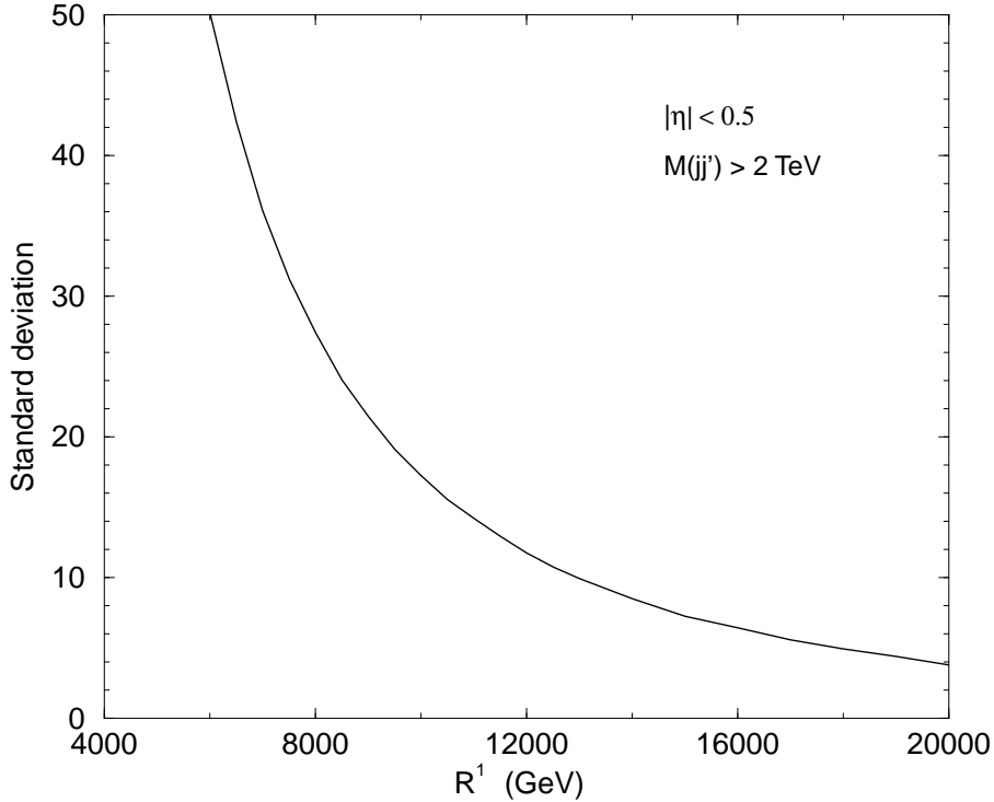
Figure 3: Number of standard deviation in number of observed dijets from the expected standard model value, due to the presence of a TeV-scale extra-dimension of compactification radius R .
