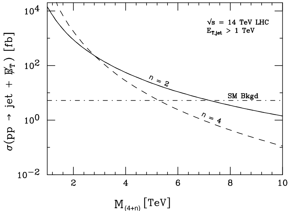
Figure 5: Missing energy due to graviton emission in the LHC experiment, as a function of the quantum gravity scale M_{(4+n)} for n large transverse dimensions, together with the Standard model background.
