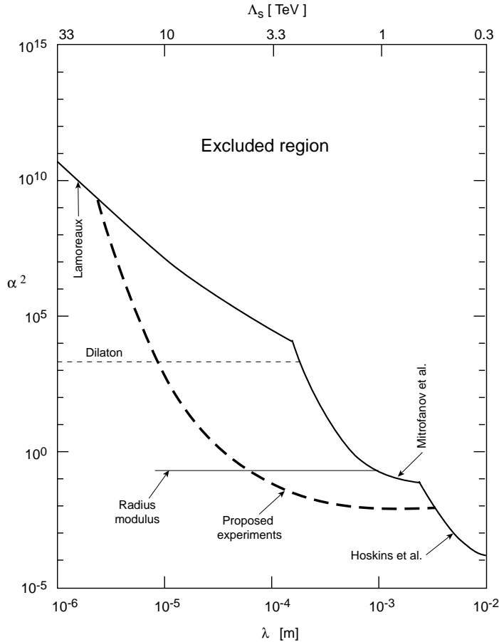
Figure 6: Strength of the modulus force relative to gravity ( \alpha^2 ) versus its Compton wavelength ( \lambda ).
