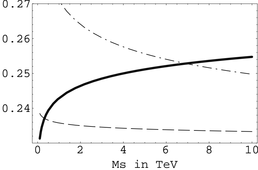
Figure 7: The experimental value of \sin^2 \theta_W (thick curve), together with the theoretical predictions (77) with c_3 = -1/3 (dashed line) and (78) with c_3 = 2/3 (dotted-dashed), are plotted as functions of the string scale M_s .
