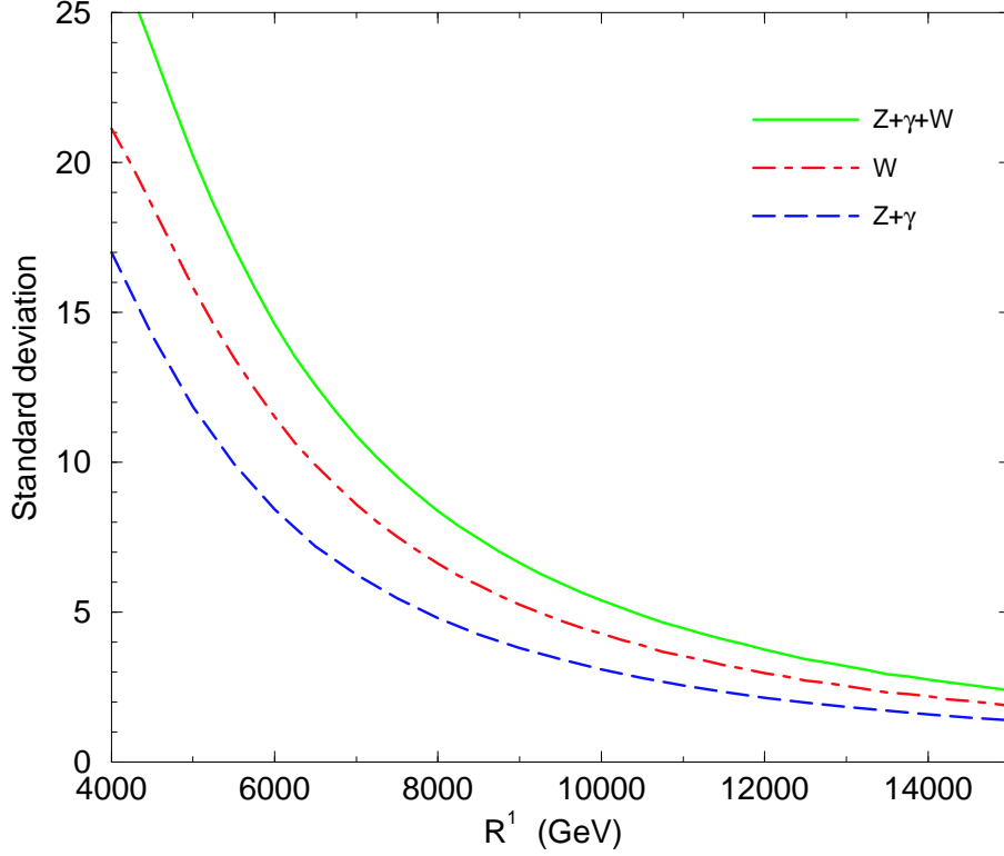
Figure 2: Number of standard deviation in the number of l^+l^- pairs and \nu_l pairs produced from the expected standard model value due to the presence of one extra-dimension of radius R .
