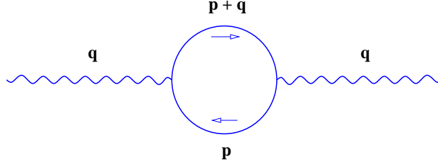
Figure 1: Generic one-loop diagram contributing to \Omega_i , with KK modes in the loop. Its value for q^2 = 0 can be read from eq.(15), (23) for one and two compact dimensions, respectively. See also Appendix A in [23].
