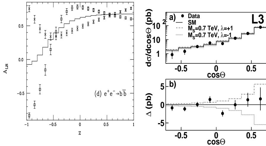
Figure 3: (Left) Distribution of the angular dependence ( z = \cos\theta ) of the polarized Left-Right asymmetry in e^+e^- \rightarrow b\bar{b} with \sqrt{s} = 500 GeV, taking M_D = 1.5 TeV and \lambda = \pm 1 . The solid histogram is the Standard Model expectation. The two sets of data points correspond to the two choices of sign for \lambda , and the error bars represent the statistics in each bin for an integrated luminosity of 75 \text{ fb}^{-1} . From (24). (Right) (a) Differential cross section for Bhabha scattering in the LEP data and for the Standard Model expectations; the modification for M_D=0.7 TeV and \lambda = \pm 1 is as indicated. (b) The difference of the above with the Standard Model prediction. From (19).
