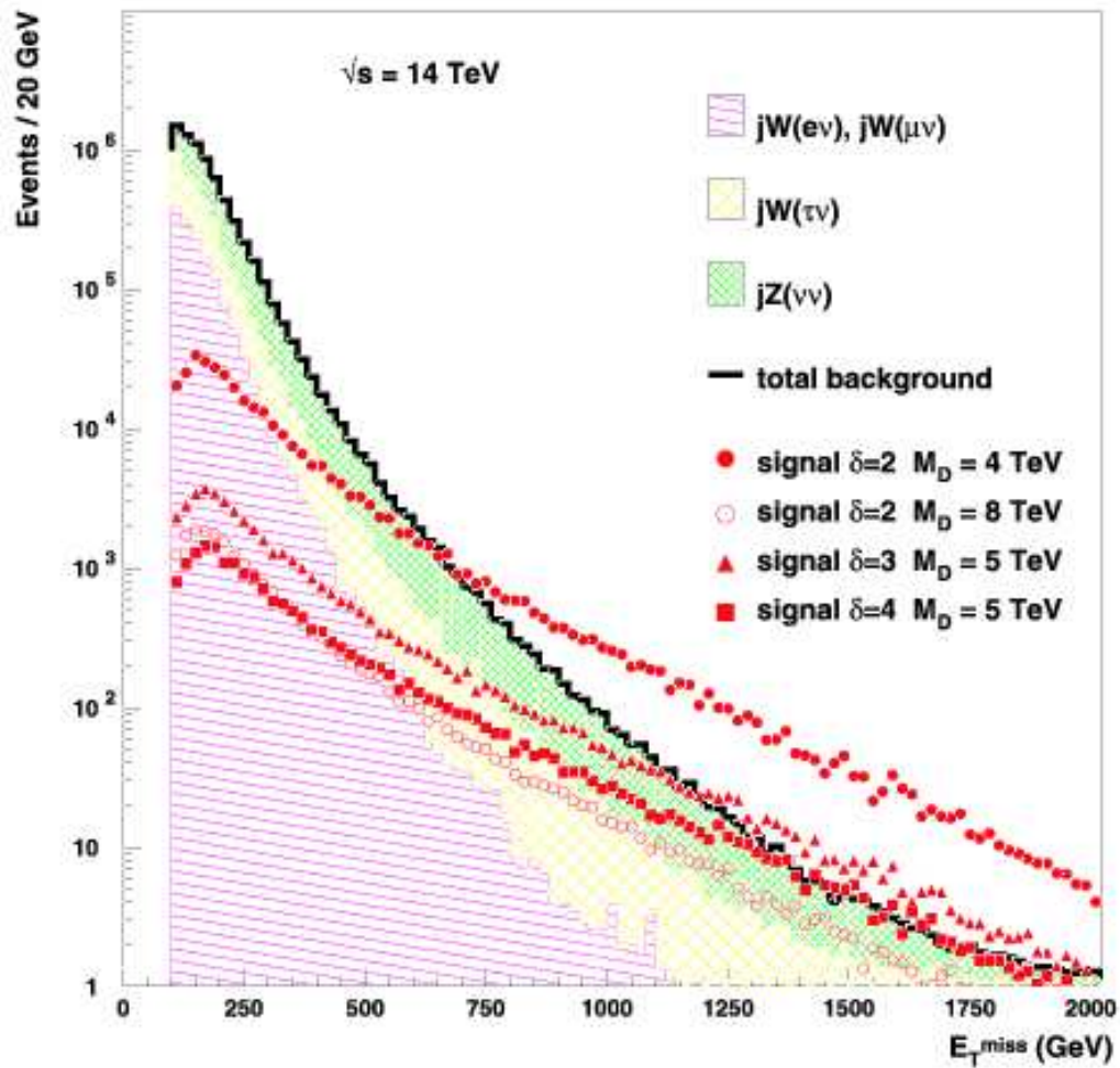
Figure 2: Distribution of the missing transverse energy in background events and signal events for 100 \text{ fb}^{-1} . The contribution of the three principal Standard Model background processes is shown as well as the distribution of the signal for several values of \delta and M_D . From (22).
