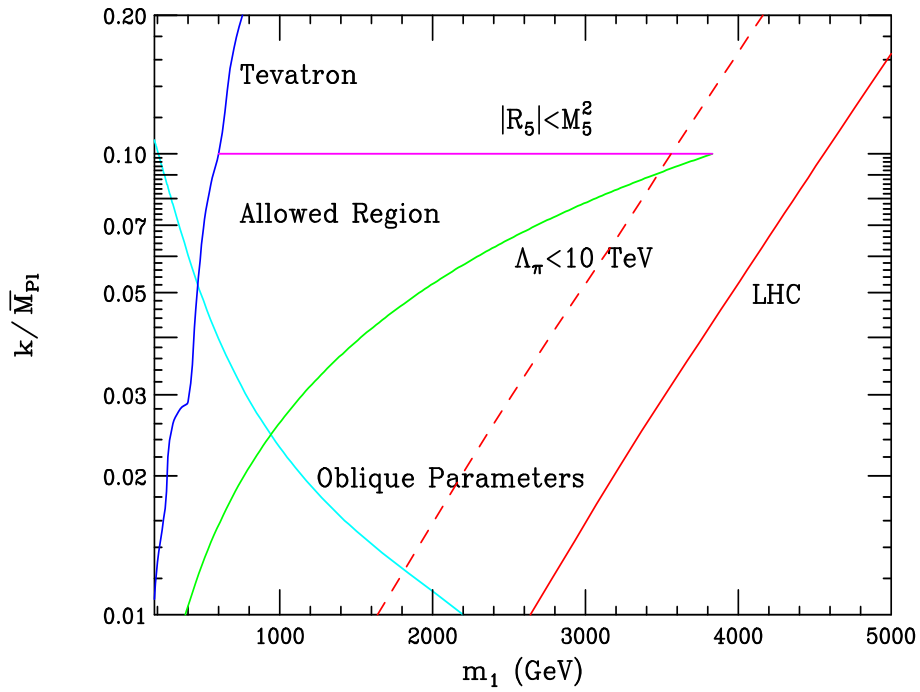
Figure 6: Summary of experimental and theoretical constraints on the Randall-Sundrum model in the two-parameter plane k/\overline{M}_{\text{Pl}} - m_1 , for the case where the Standard Model fields are constrained to the TeV-brane. The allowed region lies in the center as indicated. The LHC sensitivity to graviton resonances in the Drell-Yan channel is represented by the diagonal dashed and solid curves, corresponding to 10 and 100 \text{fb}^{-1} of integrated luminosity, respectively. From (38).
