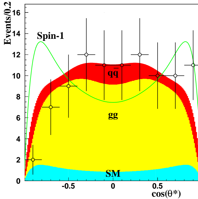
Figure 5: The angular distribution of “data” at the LHC from Drell-Yan production of the first graviton KK excitation with m_1 = 1.5 TeV and 100 \text{ fb}^{-1} of integrated luminosity. The stacked histograms represent the Standard Model contributions, and gg and q\bar{q} initiated graviton production as labeled. The curve shows the expected distribution from a spin-1 resonance. From (36).
