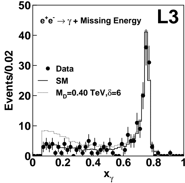
Figure 1: Distribution of the ratio of the photon energy to the beam energy for single photon events at LEP with \sqrt{s}=183 GeV. The data and expectations from the Standard Model for this reaction are indicated as labeled. The effect of real graviton production with six extra spatial dimensions and M_D = 0.4 TeV is also shown. From (19).
