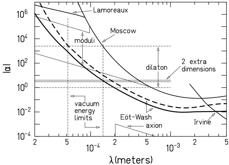
Figure 7: 95% confidence level upper limits on the strength \alpha (relative to Newtonian gravity) as a function of the range \lambda of additional Yukawa interactions. The region excluded by previous experiments (55, 56, 61) lies above the curves labeled Irvine, Moscow and Lamoreaux, respectively. The most recent results (60) correspond to the curves labeled Eöt-Wash. The heavy dashed line is the result from Ref. (60), the heavy solid line shows the most recent analysis that uses the total data sample.
