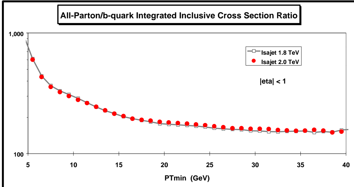
Plot shows the inclusive cross section \sigma(\text{PT} > \text{PT}_{\text{min}}, |\eta| < 1) for all partons (divided by 2) divided by \sigma(\text{PT} > \text{PT}_{\text{min}}, |\eta| < 1) for b-quarks at 1.8 TeV and 2.0 TeV.
