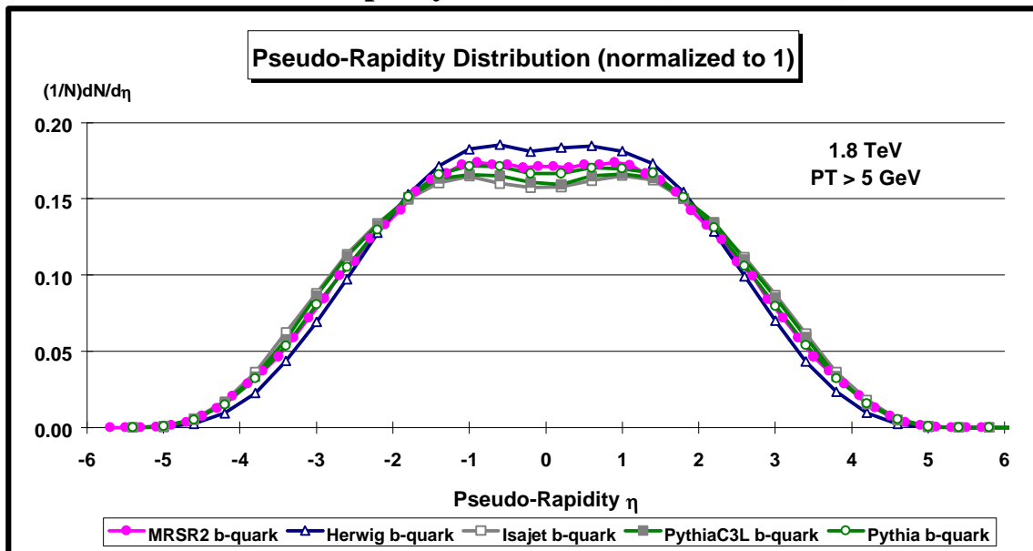
Plot shows (1/N)dN/d\eta (normalized to 1) for b-quarks at 1.8 TeV (PT > 5 GeV).
