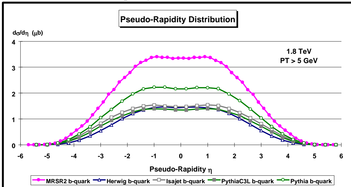
Plot shows d\sigma/d\eta (in \mu\text{b} ) for b-quarks at 1.8 TeV (PT > 5 GeV).
