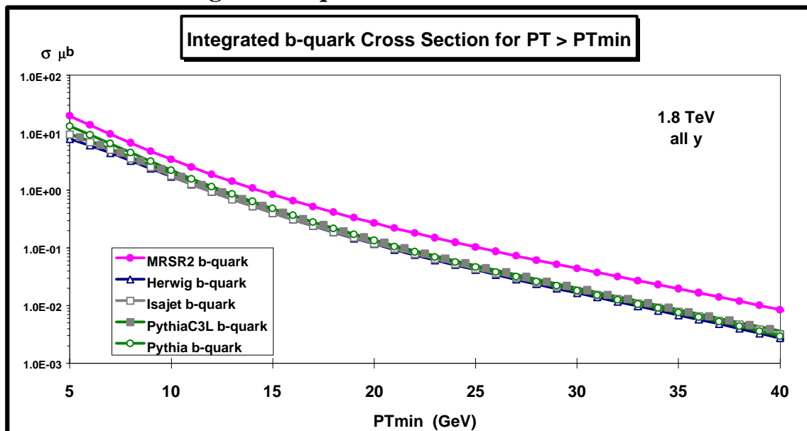
Plot shows \sigma(PT > PT_{min}) (in \mu b ) for b-quarks at 1.8 TeV (all Y).
