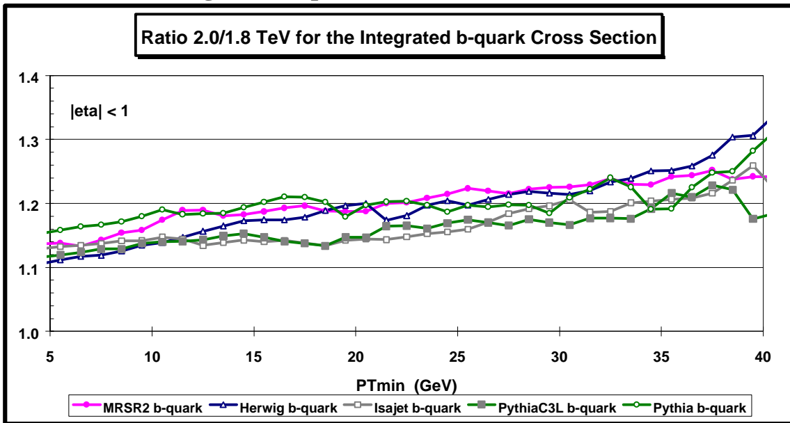
Plot shows the 2.0/1.9 TeV ratio of \sigma(PT > PT_{min}) for b-quarks ( |\eta| < 1 ).
