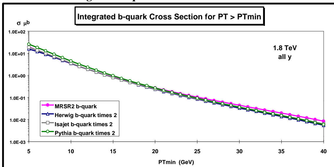
Plot shows \sigma(PT > PT_{min}) (in \mu b ) for b-quarks at 1.8 TeV (all Y). Herwig, Isajet, and Pythia have been increased by a factor of two .
