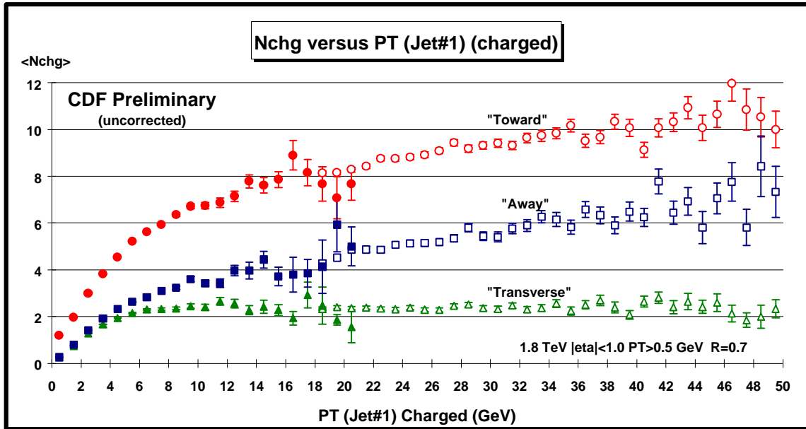
Plot 4: “Toward”, “Transverse”, “Away” \langle N_{chg} \rangle vs PT(charged jet#1):
