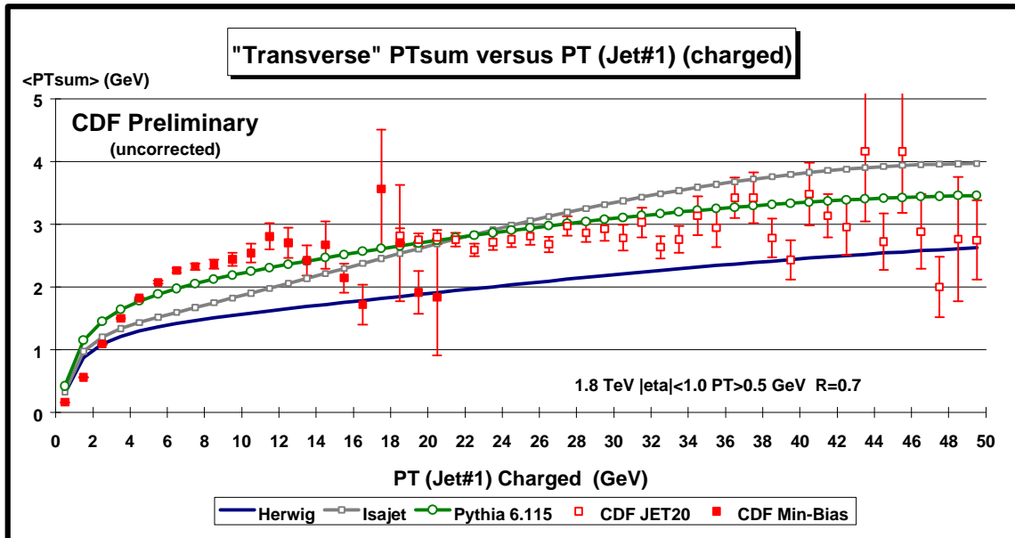
Plot 8: "Transverse" \langle PT_{sum} \rangle vs PT(charged jet#1):
