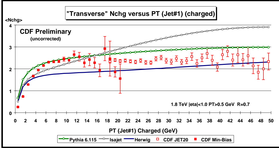
Plot 7: "Transverse" \langle N_{chg} \rangle vs PT(charged jet#1):
