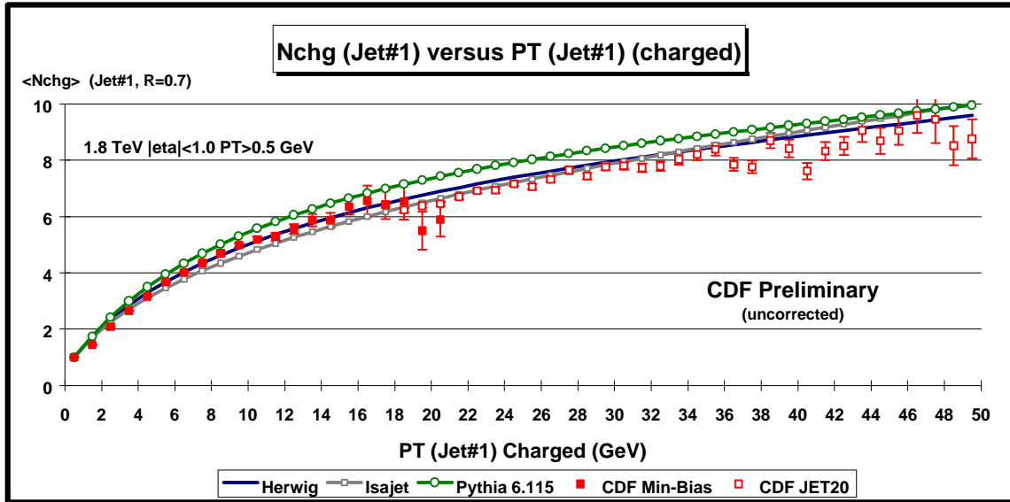
Plot 1: \langle N_{\text{chg}}(\text{jet}\#1) \rangle vs PT(\text{charged jet}\#1) :
