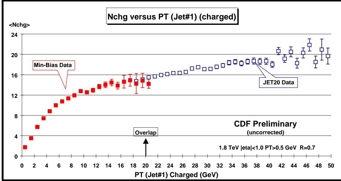
Plot 3: \langle N_{chg} \rangle vs PT(charged jet#1):
