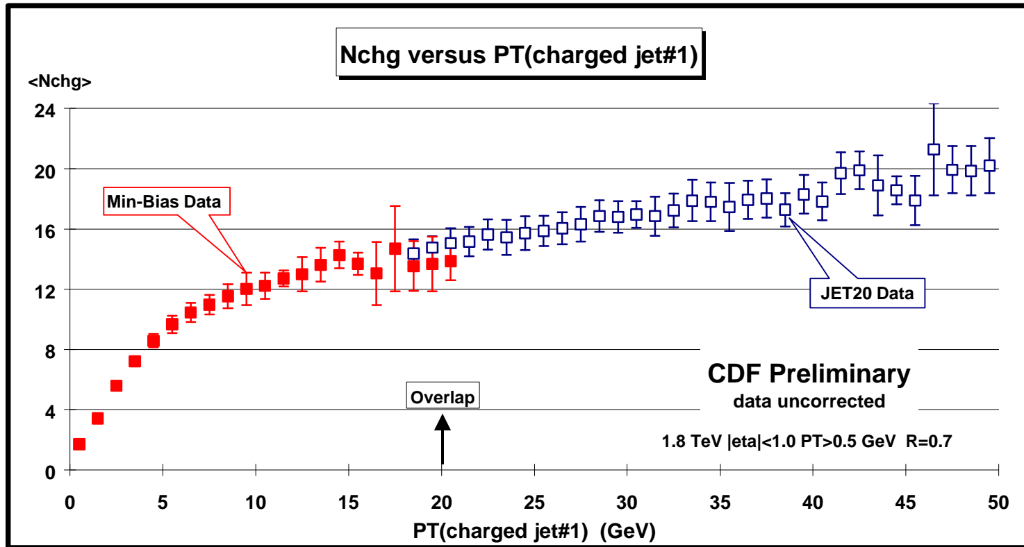
Plot shows the average number of charged particles ( PT > 0.5 GeV, |\eta| < 1 including jet#1) as a function of the PT of the leading charged jet . The errors on the (uncorrected) data include both statistical and correlated systematic uncertainties.
