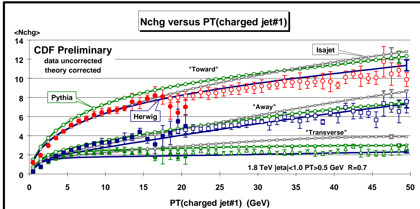
Plot 6: “Toward”, “Transverse”, “Away” \langle N_{\text{chg}} \rangle vs PT(\text{charged jet}\#1) :
