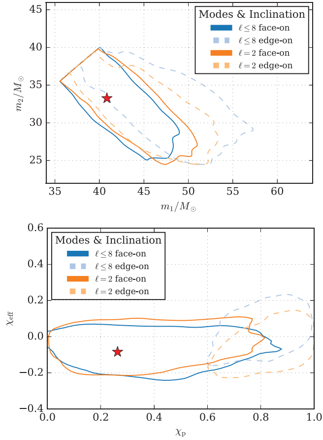
Figure 6. Results for processing NR injections (SXS : BBH : 0308) with face-on or edge-on inclination ( \theta_{\text{IN}} = 6^\circ and 84^\circ , respectively) and either including higher harmonics up to \ell = 8 (compare with figure 4) or just the \ell = 2 modes in the mock signal. All injections are performed at fiducial polarization angle \psi = 82^\circ . The precessing IMRPhenom model is used as the template waveform. We show two-dimensional 90% credible regions for component masses and effective spins.
