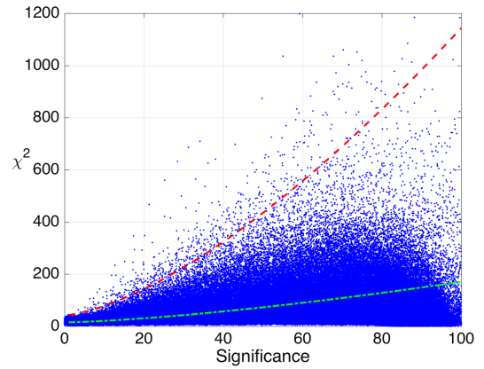
FIG. 8. Same as Fig. 7 for 320000 injections in the 100–200 Hz band. The false dismissal rate is 0.21%.
