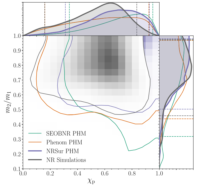
Figure 8. Posterior probability density for the precession spin parameter \chi_p and mass ratio from the direct comparison of NR simulations with GW190521 (gray tiles, and gray contour showing 90% confidence area). For comparison, shown here are the 90% bounds on these parameters from the three waveform models.
