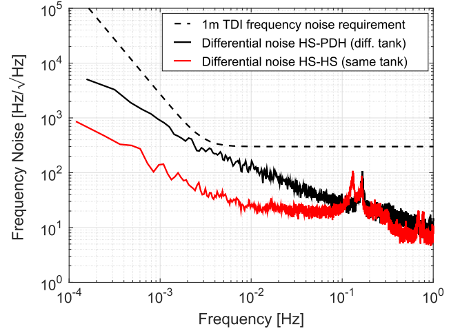
FIG. 7 (color online). Frequency stability of the HS stabilized lasers. Shown is the frequency noise of the beat between the two HS test systems, as well as the beat between the 27 cm cavity laser and an independently PDH-stabilized UFLIS reference laser. The LISA TDI requirement (1) was added as a dashed line. The peaklike features between 0.1 and 0.2 Hz emerge at the crossover between piezo- and laser crystal temperature feedback due to the limited resolution of the D/A conversion in the temperature feedback.
