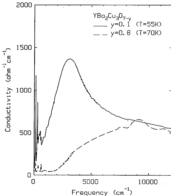
FIG. 2. The frequency-dependent conductivity of superconducting \text{YBa}_2\text{Cu}_3\text{O}_{6.9} at 55 K and of nonsuperconducting \text{YBa}_2\text{Cu}_3\text{O}_{6.2} at 70 K, as determined by Kramers-Kronig analysis of the reflectance.
