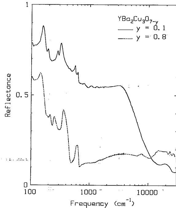
FIG. 1. Reflectance of superconducting \text{YBa}_2\text{Cu}_3\text{O}_{6.9} (at 105 K) and of nonsuperconducting \text{YBa}_2\text{Cu}_3\text{O}_{6.2} (at 300 K). Note the logarithmic frequency scale.
