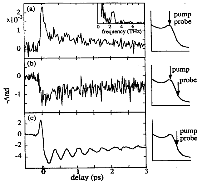
FIG. 2. Time-dependent nonlinear absorption measured at wavelengths of (a) 602 nm, (b) 602 nm (pump) and 626 nm (probe), and (c) 616 nm. The inset shows the power spectrum of the data of (a). The excitation and probe wavelengths are indicated on the 1s_e - 1s_h absorption resonance.
