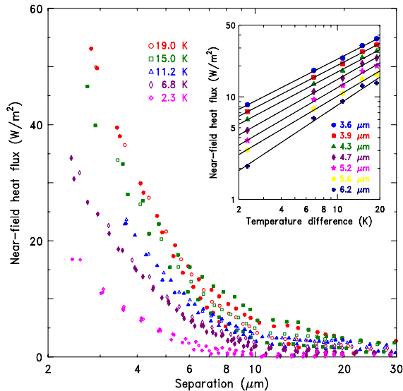
FIG. 4 (color online). Near-field heat flux vs distance for multiple temperature differences and multiple runs. (One run is shown with open symbols and other runs with filled symbols.) The inset shows the near-field heat flux vs temperature difference for several specific separation distances.
