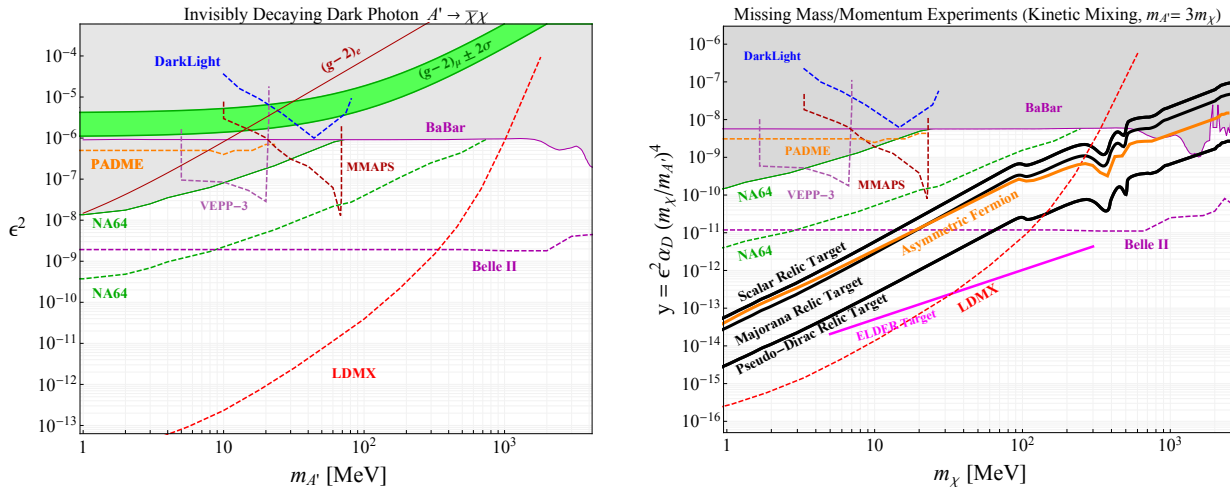
FIG. 18: Current constraints (shaded regions) and sensitivity estimates (dashed lines) on the SM-mediator coupling \epsilon = g_{\text{SM}}/e , for various experiments based on the missing mass, missing energy and missing momentum approaches. The green band show the values required to explain the muon (g-2)_\mu anomaly [56]. Right: Corresponding curves on the parameter y , plotted alongside various thermal relic target. These curves assumes m_{A'} = 3m_\chi and \alpha_D = 0.5 . For larger mass ratios or smaller values of \alpha_D , the experimental curves shift downward, but the thermal relic target remains invariant. The asymmetric DM and ELDER targets (see text) are also shown as solid orange and magenta lines, respectively. Courtesy G. Krnjaic.
