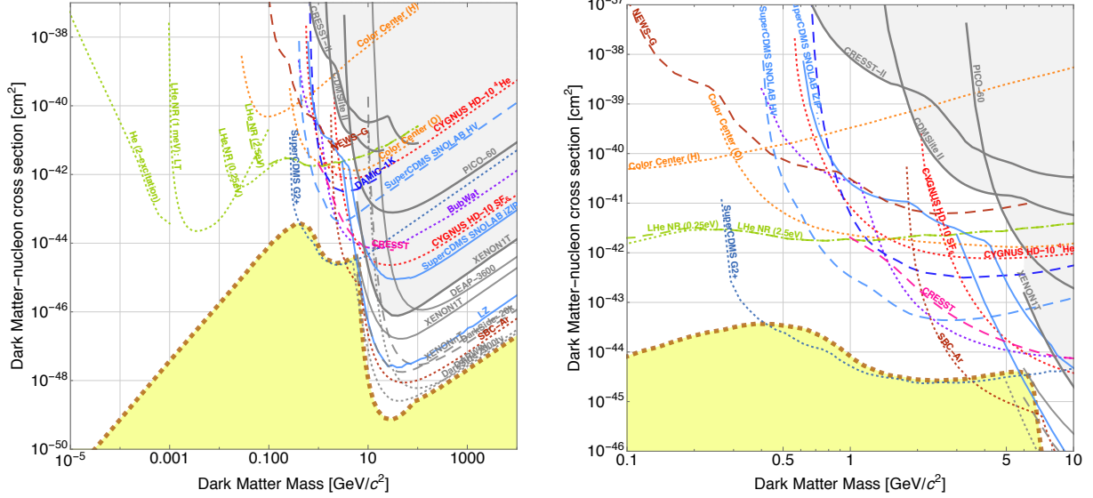
FIG. 8: Left: Constraints and projections (90% c.l.) for the DM-nucleon scattering cross section. Thick gray lines are current world-leading constraints [111, 119, 132, 133]. Projections are shown with solid/dashed/dotted lines indicating a short/medium/long timescale, respectively, with the same meaning as in Fig. 6. Blue lines denote the DoE G2 experiment projections. Yellow region denotes the WIMP-discovery limit from [134] extended to lower masses for He-based experiments. Right: As in left plot, but focused on the 100 MeV to 10 GeV DM mass range.
