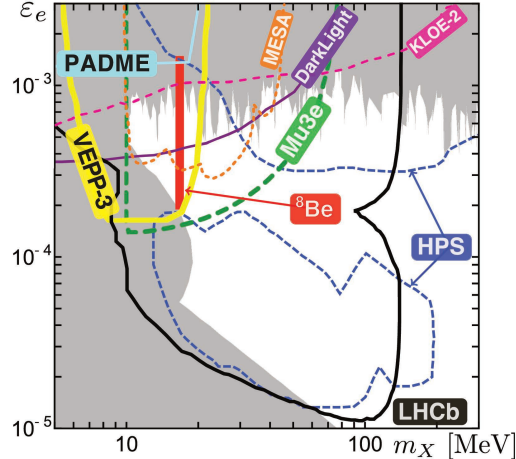
FIG. 23: The {}^8\text{Be} signal region in the (m_X, \varepsilon_e) plane, along with current constraints (gray) and projected sensitivities of the indicated future experiments. From Ref. [64].
