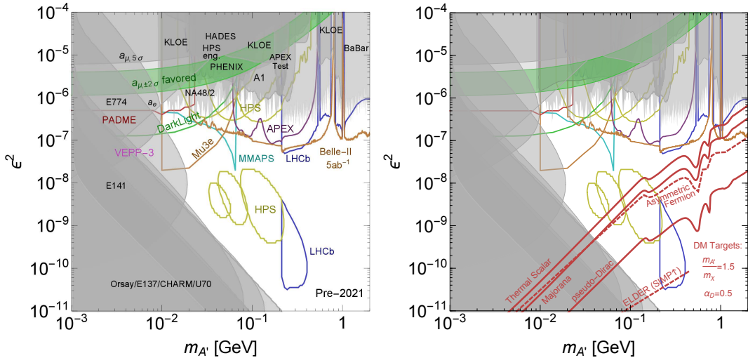
FIG. 22: Left: Constraints on visibly-decaying mediators, taken from Ref. [180]. Visible decays of the mediator dominate in the m_\chi > m_{A'} secluded annihilation regime. Existing constraints are shown in shaded, while projected sensitivities of currently running or upcoming probes are shown in solid lines. Right: Constraints on visibly-decaying mediators, together with the thermal relic (solid red lines), asymmetric DM and ELDER (dashed red lines) targets. The prescription m_{A'} = 1.5 m_\chi and \alpha_D = 0.5 is adopted when applicable. Courtesy R. Essig, N. Toro.
