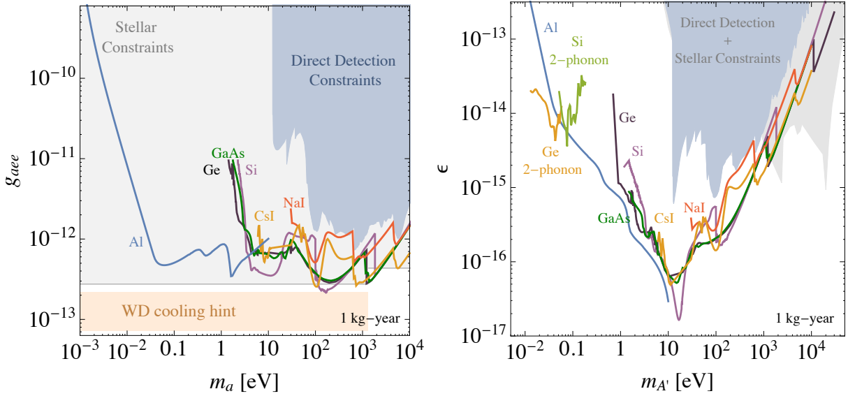
FIG. 7: Event rates for the absorption by an electron of axion-like particle (ALP) DM (left) and dark-photon ( A' ) DM (right), assuming that the ALP/ A' constitutes all the DM [89–91]. The solid colored lines show the ALP-electron coupling g_{aee} or the kinetic-mixing parameter \epsilon needed to produce 3 events for an exposure of 1 kg-year. Blue regions show constraints from WIMP direct-detection experiments [91, 103, 127–131]. Gray regions show stellar cooling constraints. In-medium effects are included for all A' constraints and projections. Shaded orange region in left plot is consistent with an ALP possibly explaining the white dwarf luminosity function.
