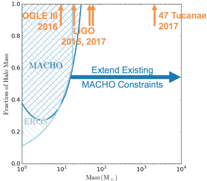
FIG. 26: Existing microlensing constraints on the fraction of the mass in the Milky Way halo that can be composed of intermediate mass MACHO dark matter. The masses of detected black holes [337–339] are indicated in orange. From Ref. [340].
