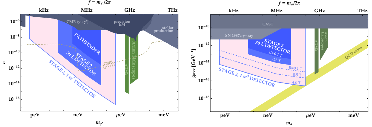
FIG. 12: Left: DM Radio sensitivity to hidden photons: upper-level constraints on photon-hidden-photon coupling \varepsilon as a function of hidden photon mass m_{\gamma'} . Right: DM Radio sensitivity to axions: upper-level constraints on axion-photon coupling g_{a\gamma\gamma} as a function of axion mass m_a and applied DC magnetic field B .
