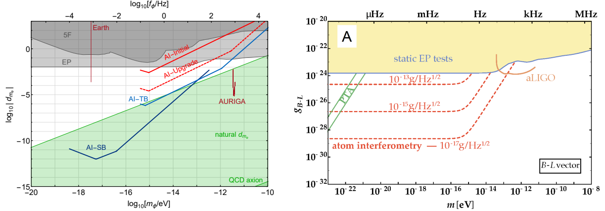
FIG. 14: Left: Sensitivity of the MAGIS-100 atom interferometer to scalar DM-electron coupling d_{m_e} measured relative to gravitational strength [154]. Right: An initial BTBAI interferometer (dashed red) will reach coupling sensitivity of 10^{-15}g/\text{Hz}^{1/2} for B-L dark matter [146]. The green curves give the range probed by the EPTA and future SKA pulsar timing arrays.
