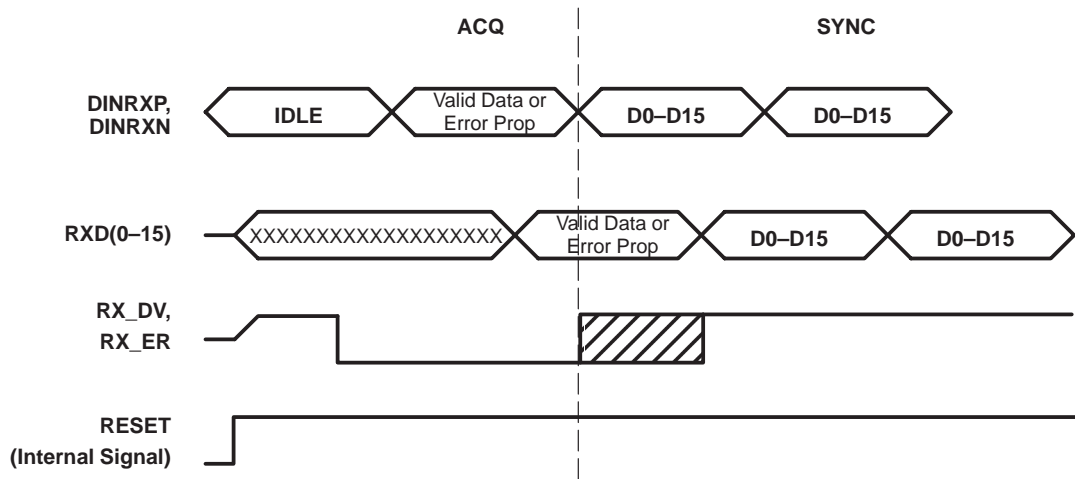
Figure 9. Receive Side Timing Diagram (Valid Data or Error Propagation)
