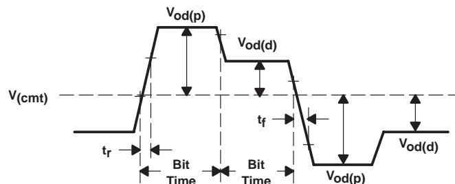
Figure 12. Differential and Common-Mode Output Voltage Definitions
